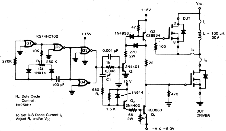
Fig. 11. Clamped Inductive Test Circuit
