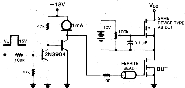
Fig. 10. Gate Charge Test Circuit.
