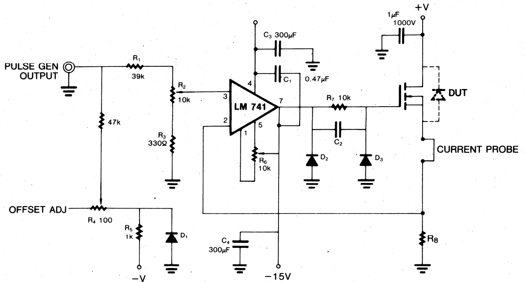
Fig. 7. Safe Operating Area Test Circuit (SOA)
