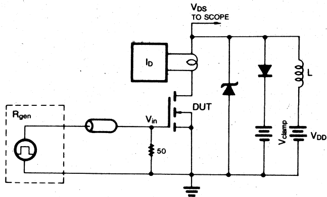
Fig. 11. Clamped Inductive Test Circuit
