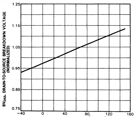
Breakdown Voltage Vs. Temperature
