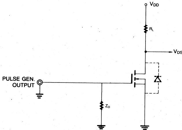
Fig. 8. Switching Time Test Circuit
