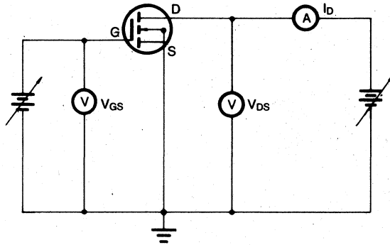
Fig. 3. Test Circuit for Drain-Source on-Resistance ( R_{DS(on)} )
