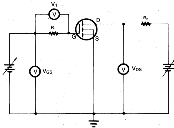
Fig. 2. Test Circuit for Gate-Source Leakage Current ( I_{GSS} )
